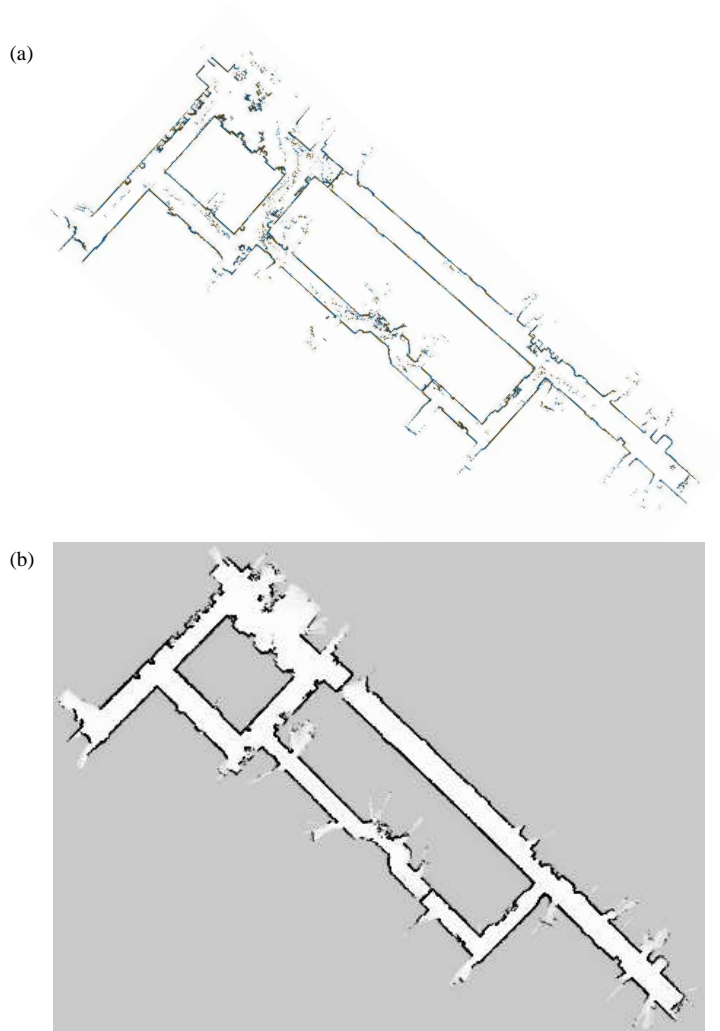
Figure 9.4 (a) Raw laser range data with correct(ed) pose information. Each dot corresponds to a detection of an obstacle. Most obstacles are static (walls etc.), but some were people that walked in the vicinity of the robot. (b) Occupancy grid map built from the data. The grey-scale indicates the posterior probability: Black corresponds to occupied with high certainty, and white to free with high certainty. The grey background color represents the prior. Figure (a) has been generated by Steffen Gutmann.
